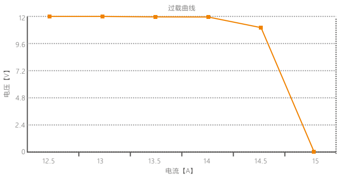
LM-150-12-G2D2
